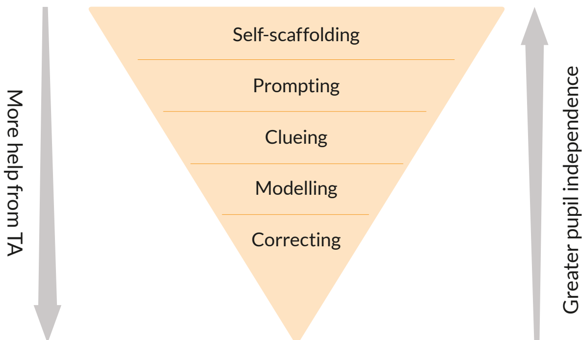
Figure 9: Scaffolding model
